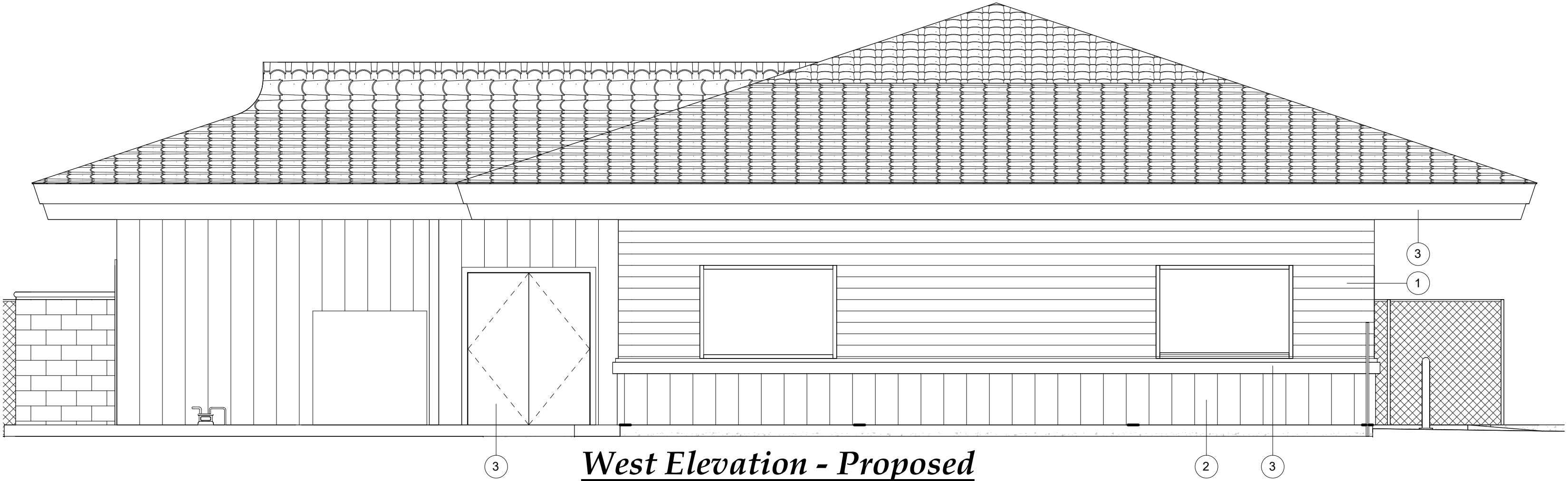
West Elevation - Proposed 1/4" = 1'-0"
