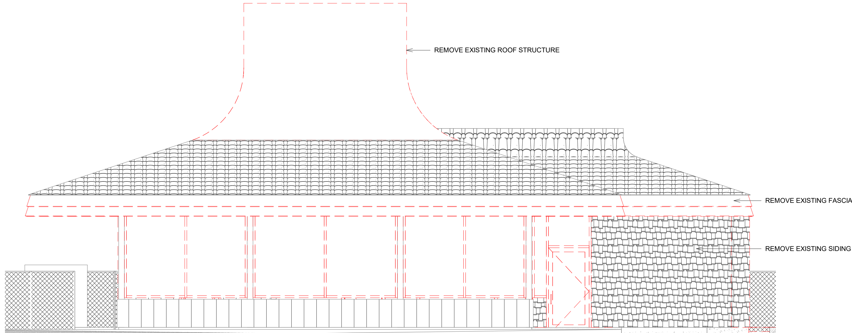
South Elevation - Existing/Demo 1/4" = 1'-0"
