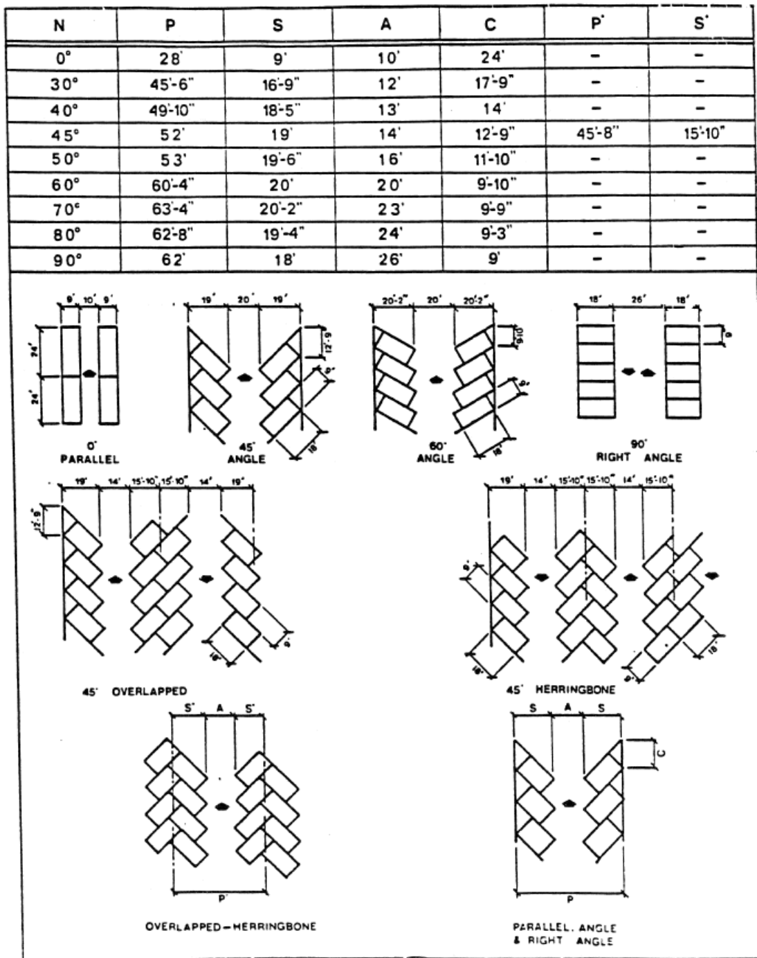
Figure 17.60--STANDARD SPACES
