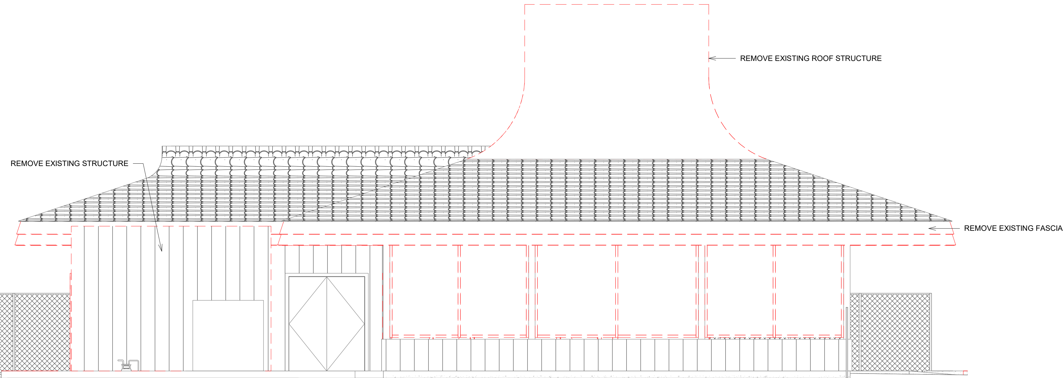
West Elevation - Existing/Demo 1/4" = 1'-0"
