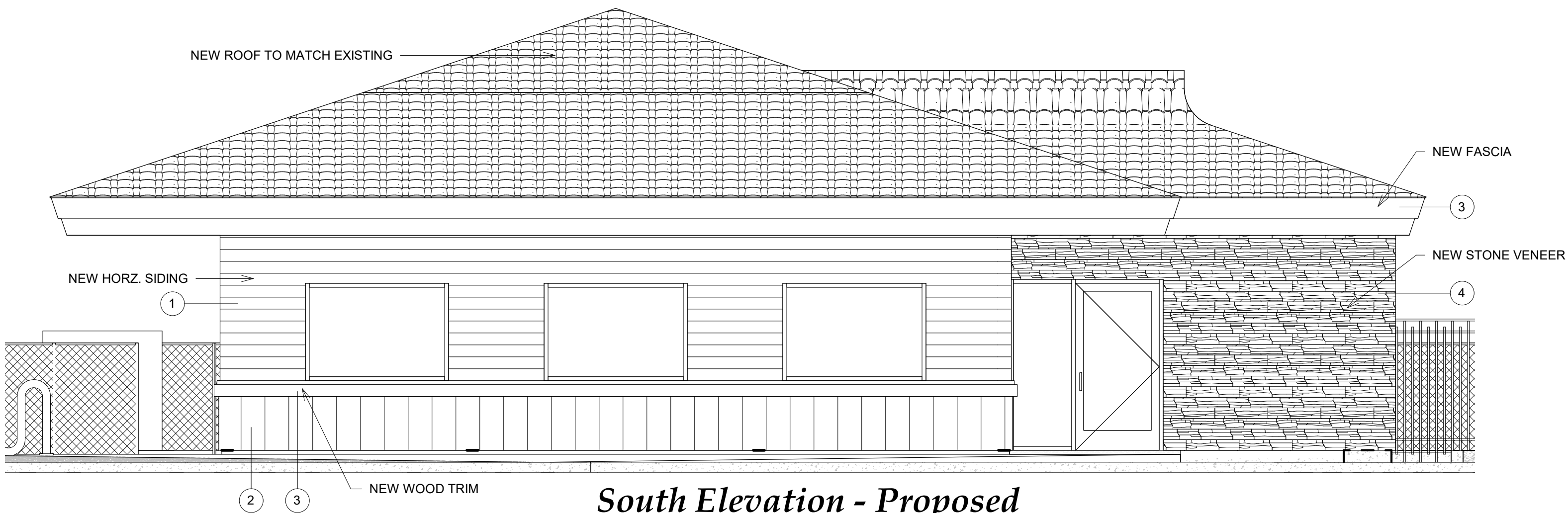
South Elevation - Proposed 1/4" = 1'-0"
