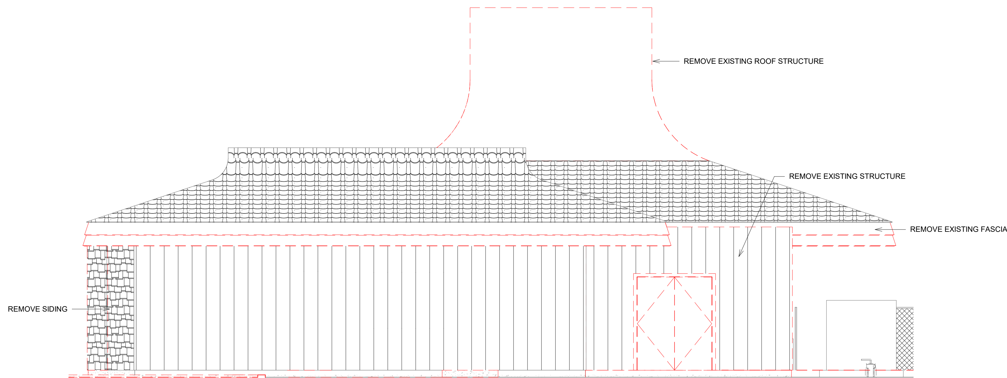
North Elevation - Existing/Demo 1/4" = 1'-0"
