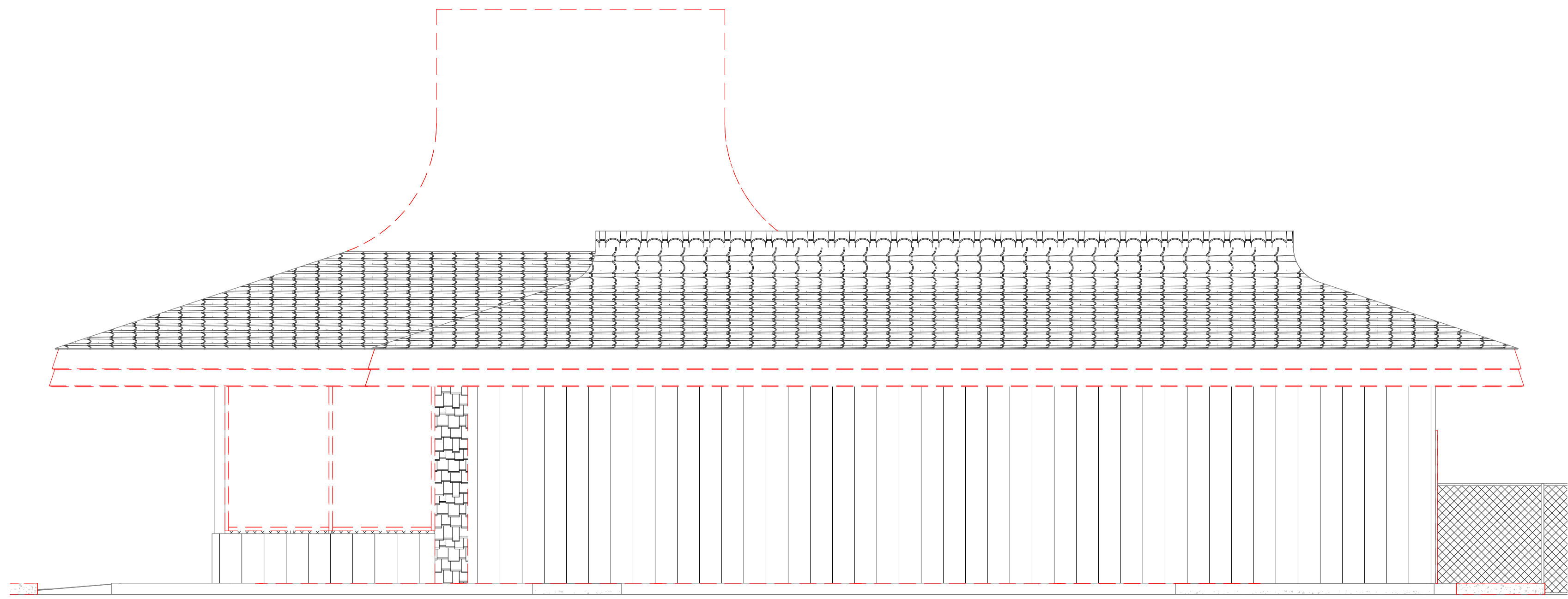
East Elevation - Existing/Demo 1/4" = 1'-0"
